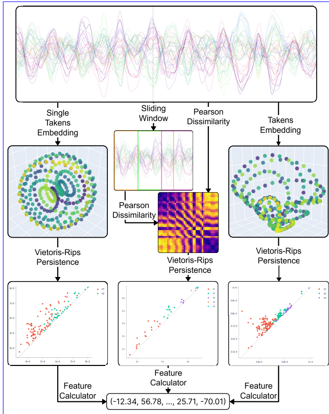
Figure 3. The scheme of the algorithm for extracting the topological features from the EEG.
