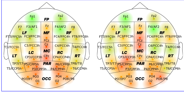
Figure 7. Feature quality scores (QSDA on the left, IV on the right) aggregated by their source electrode averaged over 30 subjects. To account for the distinctions in electrode placement during different expeditions, we merge similar electrodes from different recordings into one point on the diagram. The respective mappings are indicated in the labels of such points using the ‘/’ symbol.
