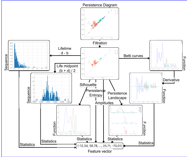
Figure 4. The scheme of the pipeline to vectorize the persistence diagrams.
