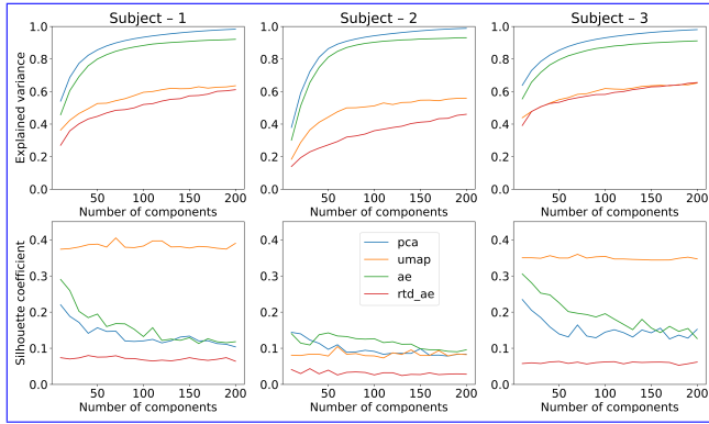
Figure 5. Explained variance (top) and achieved resulting quality (bottom) of four dimensionality reduction algorithms for objects subjects 1 (left), 2 (middle), and 3 (right).
